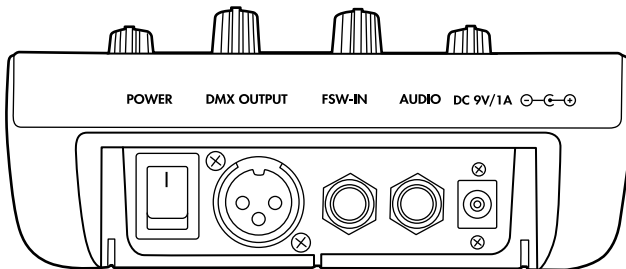
Back Panel
